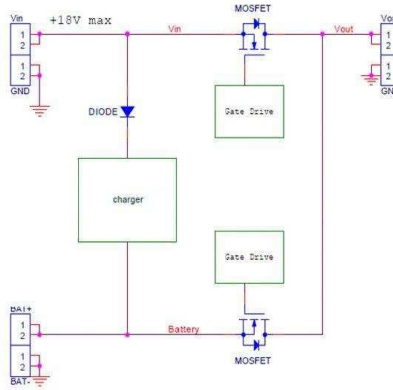
Fig 1.1 picoUPS-120-ATV block diagram
