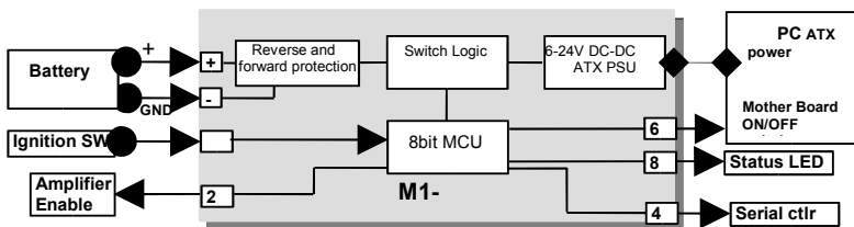
1.2 M3-ATX Connection diagram
